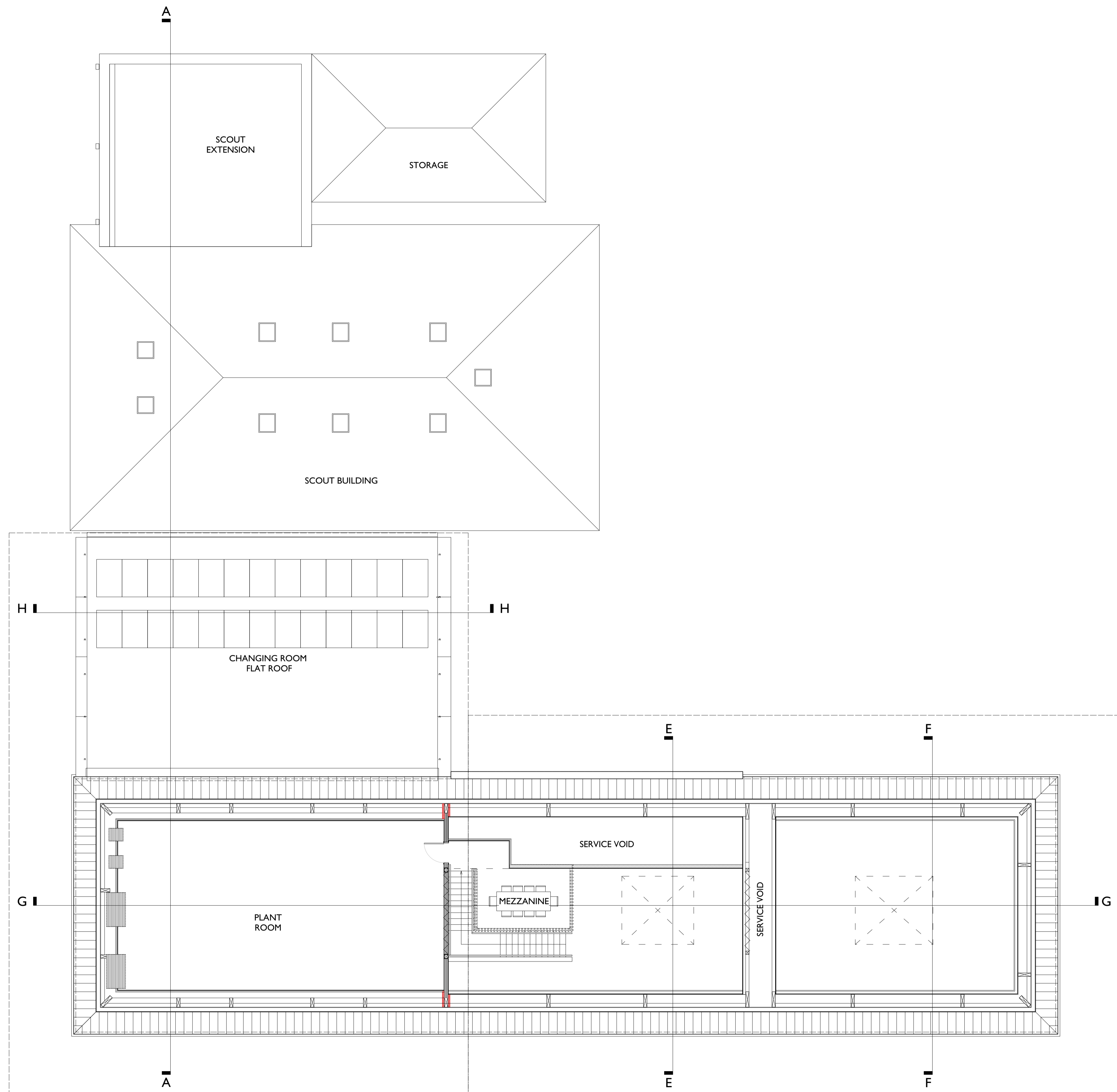
First Floor Plan - Zone 2 21_052 310
